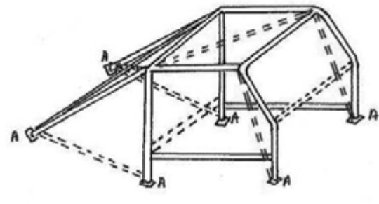
b) Diagonal(s) across Back Stays
