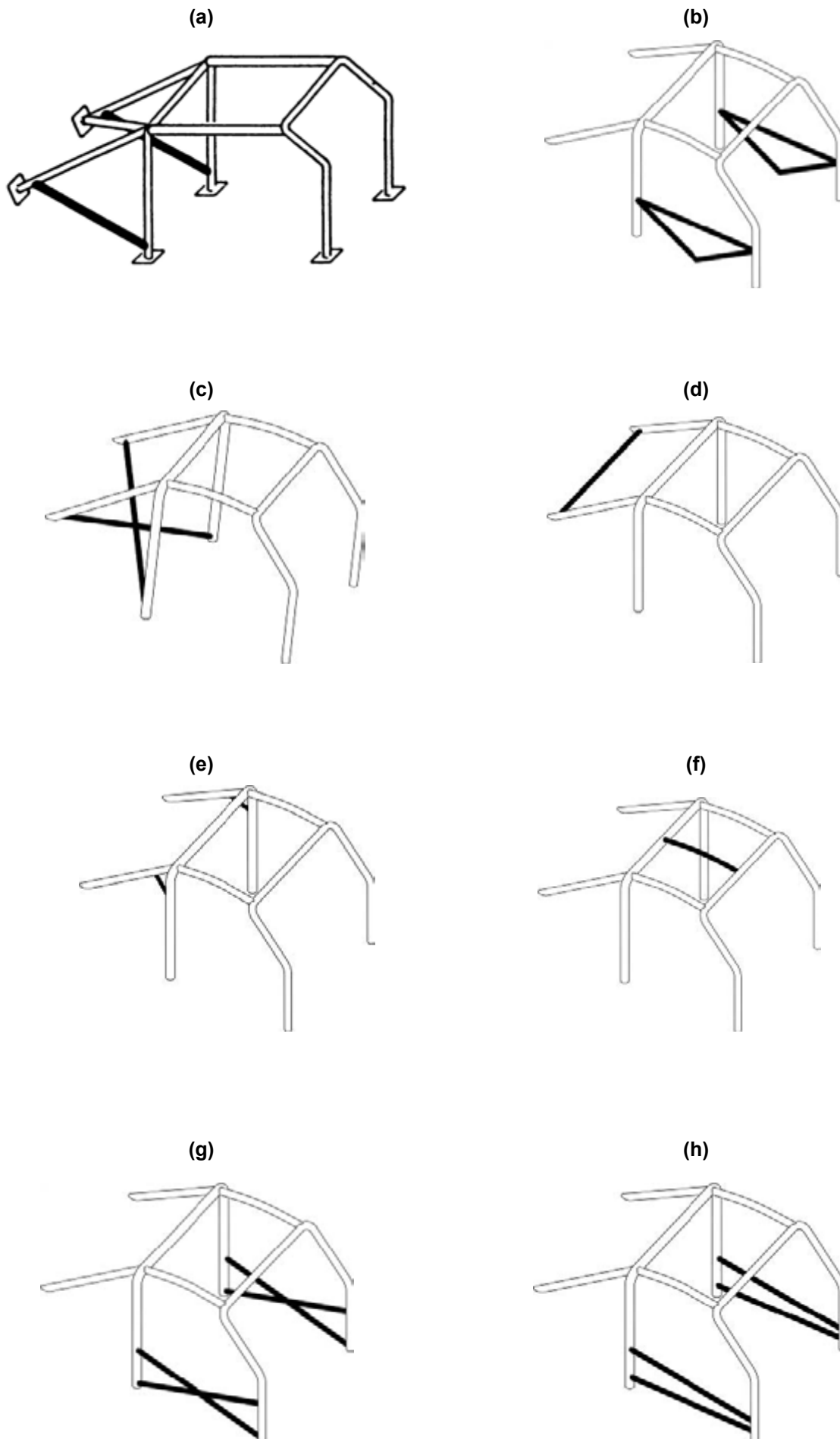
Diagram 21 Optional Reinforcing Members [6]
